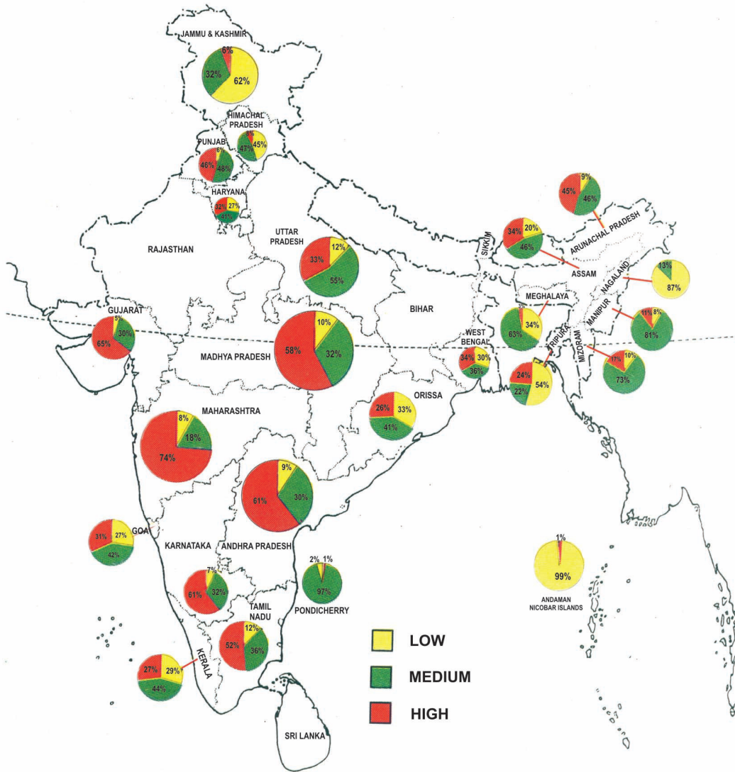
Figure 6: POTASSIUM FERTILITY STATUS OF SOILS OF INDIAN STATES
